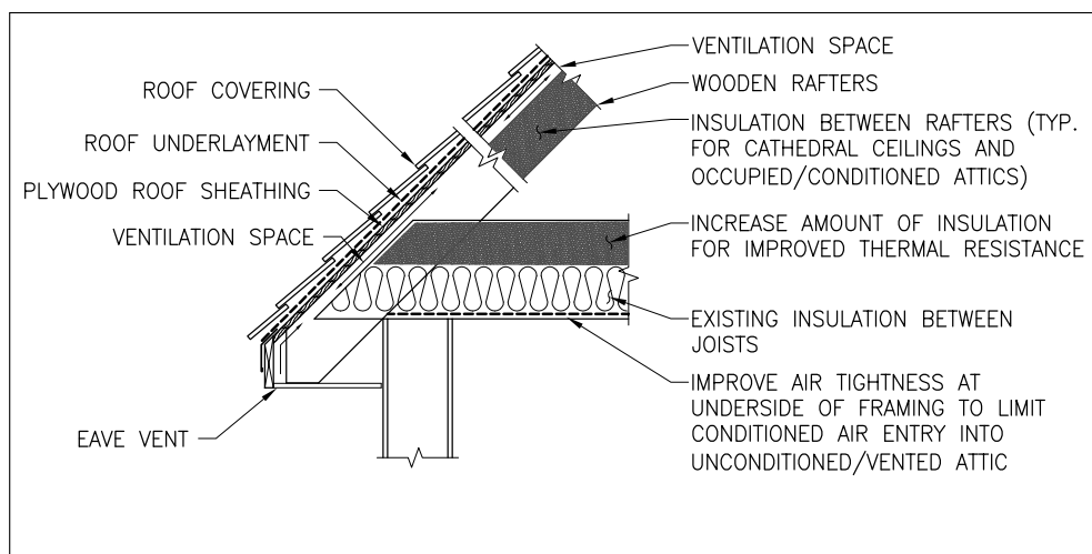
ROOF EAVE VENT
