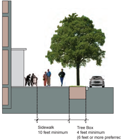
Typical Commercial Cross-Section (Outside of Downtown Area)
