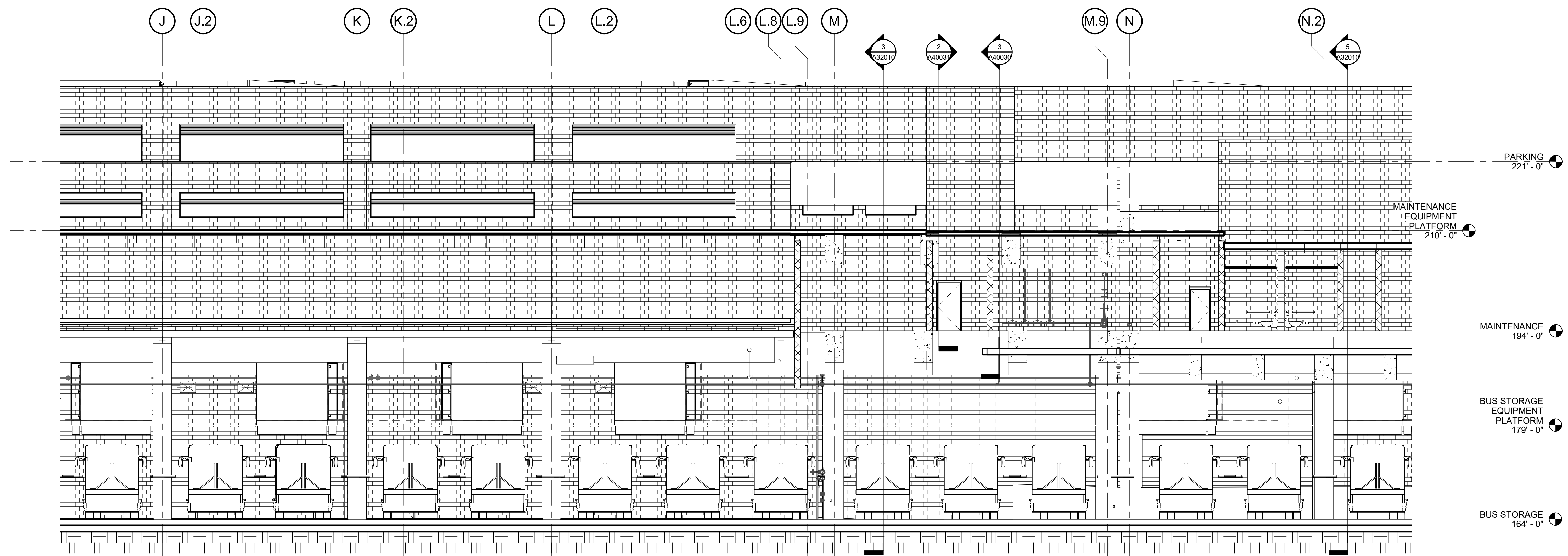
Section 29 - Callout 3 1/8" = 1'-0"
