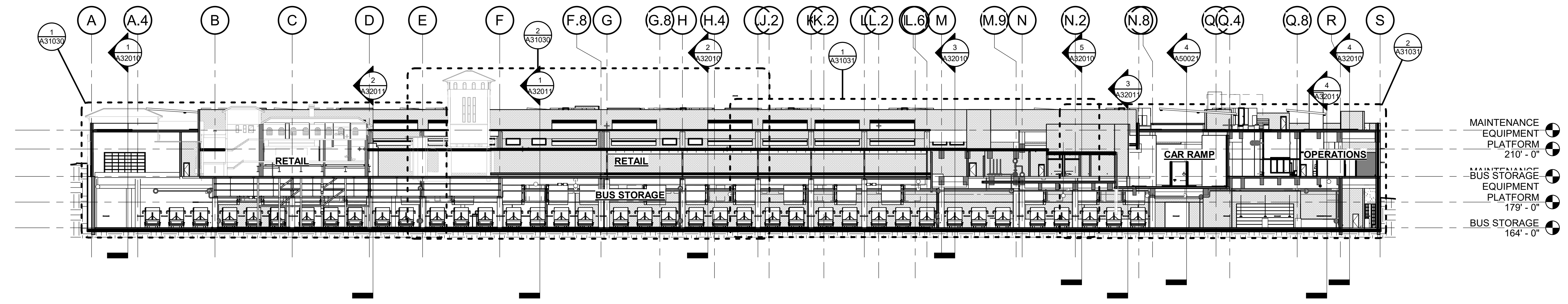
2 BUILDING SECTION OVERALL- NS4 A01000 1/32" = 1'-0"
