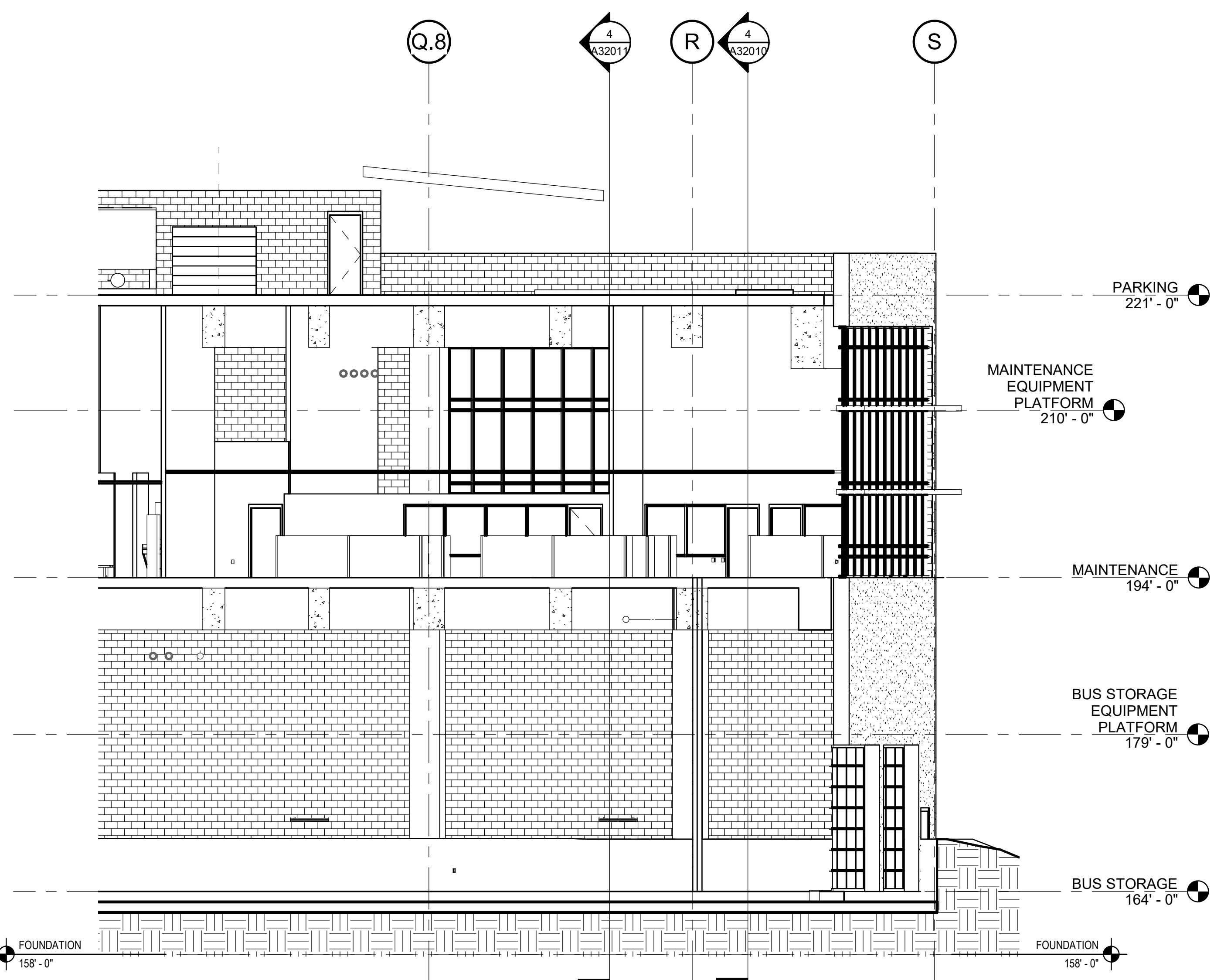
Section 27 - Callout 4 1/8" = 1'-0"
