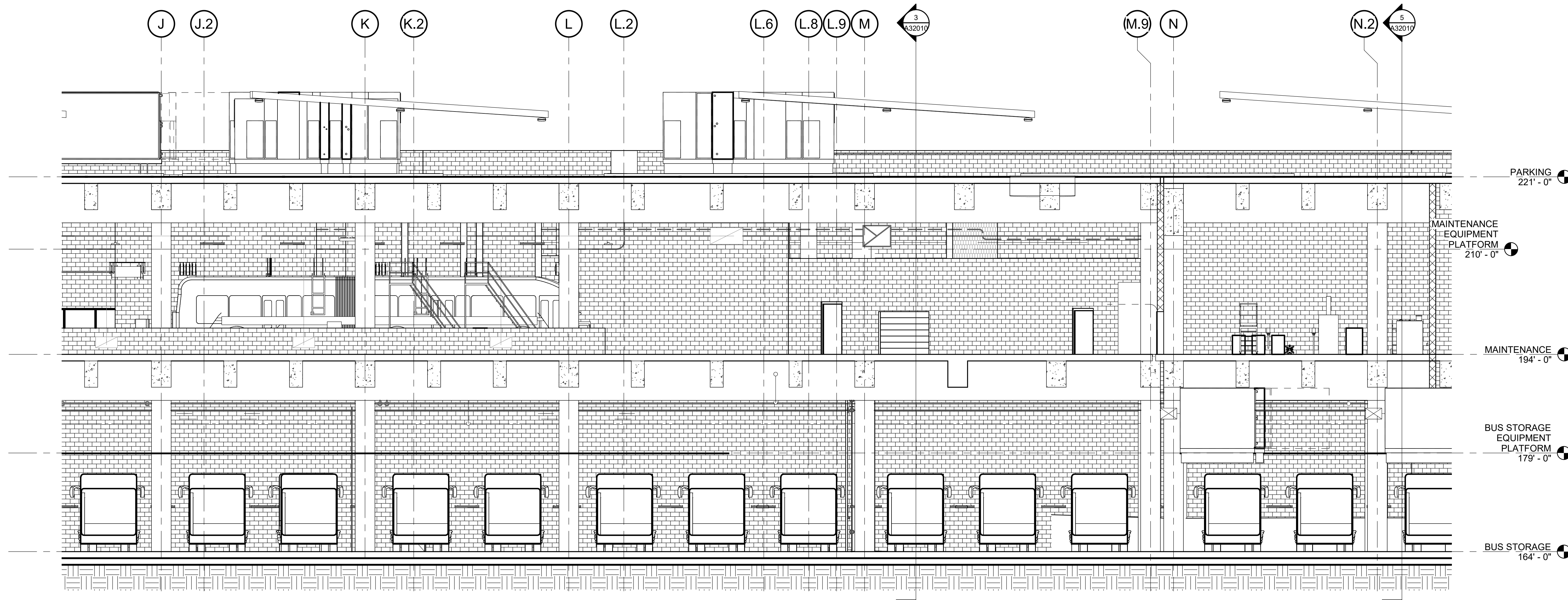
Section 28 - Callout 3 1/8" = 1'-0"
