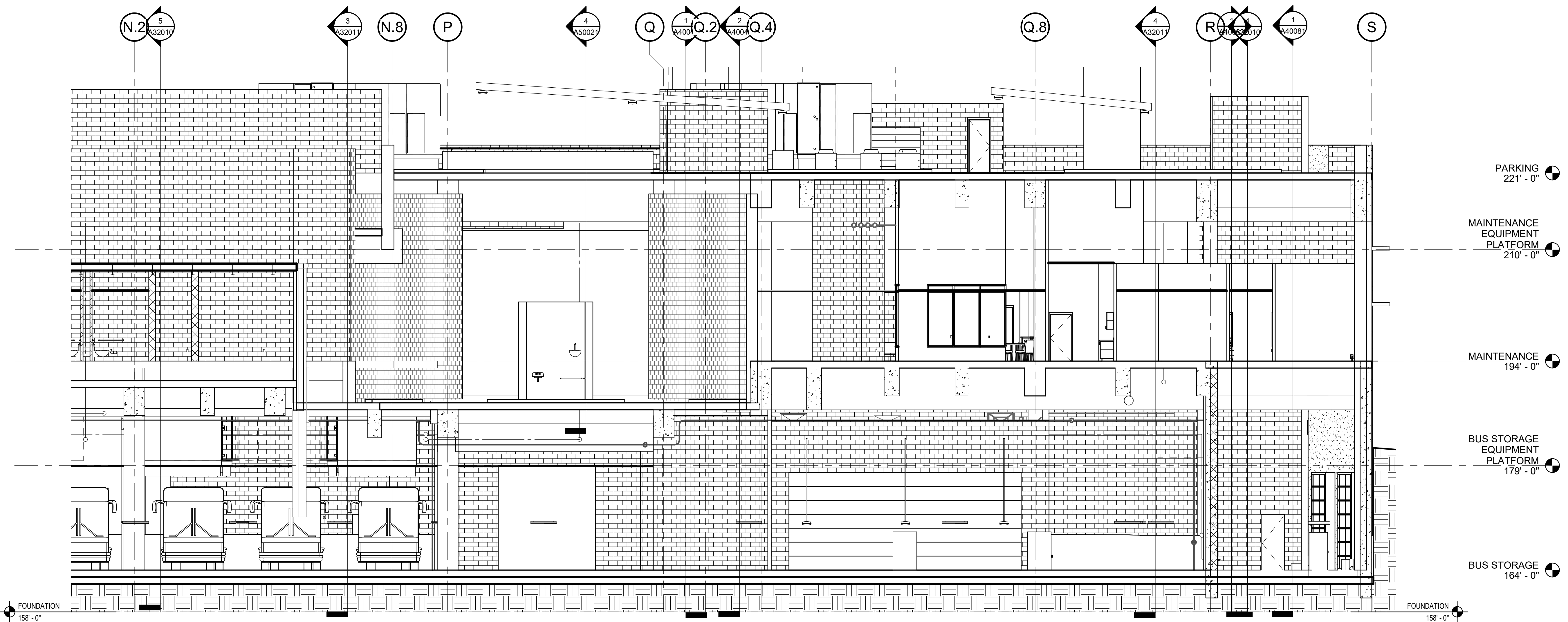
Section 29 - Callout 4 1/8" = 1'-0"
