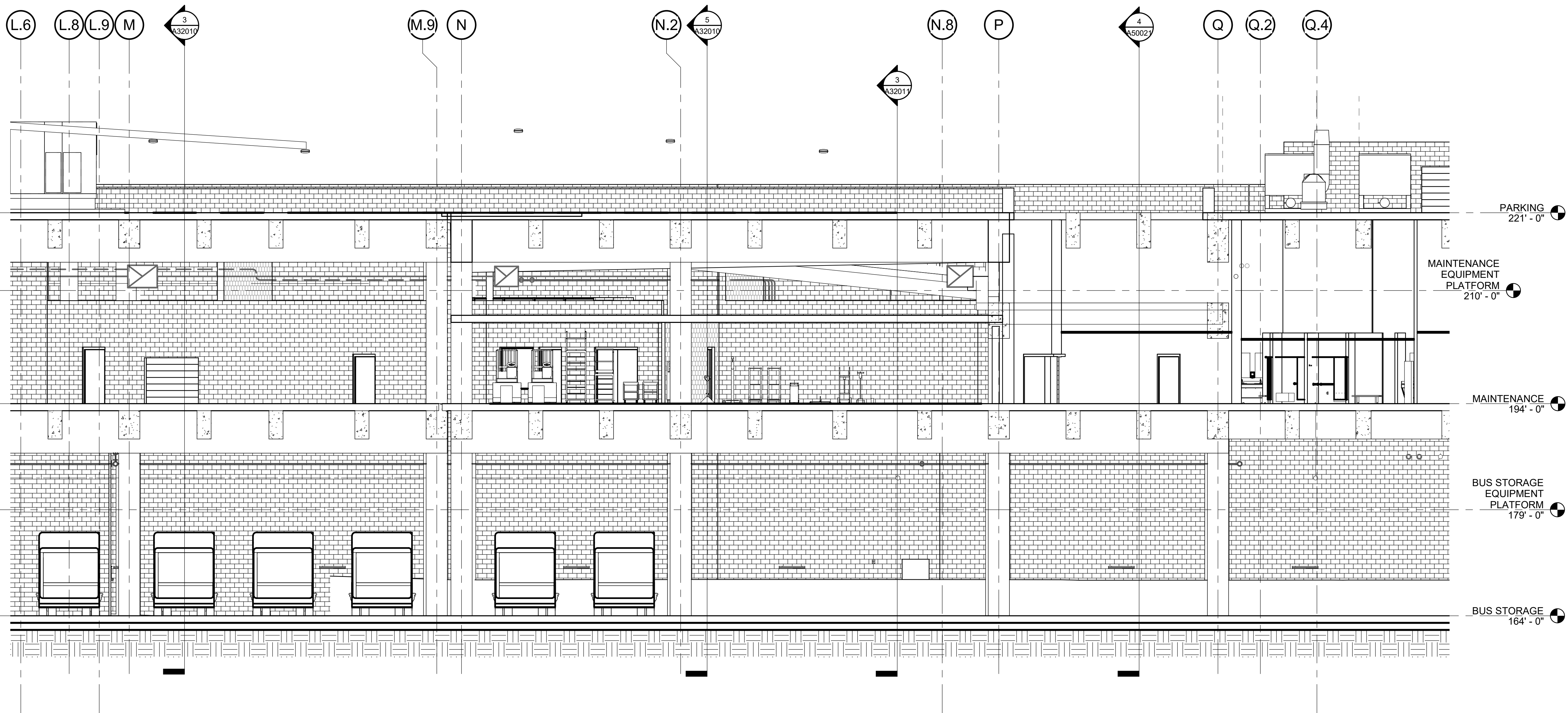
Section 27 - Callout 3 1/8" = 1'-0"
