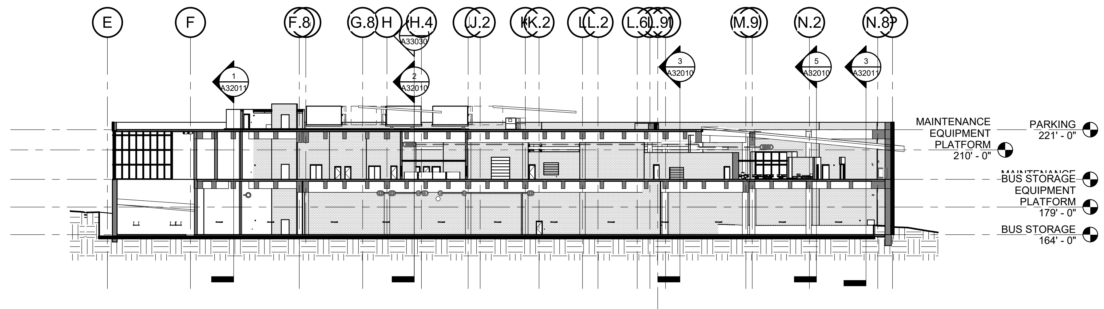
1 BUILDING SECTION OVERALL- NS5 A01000 1/32" = 1'-0"
