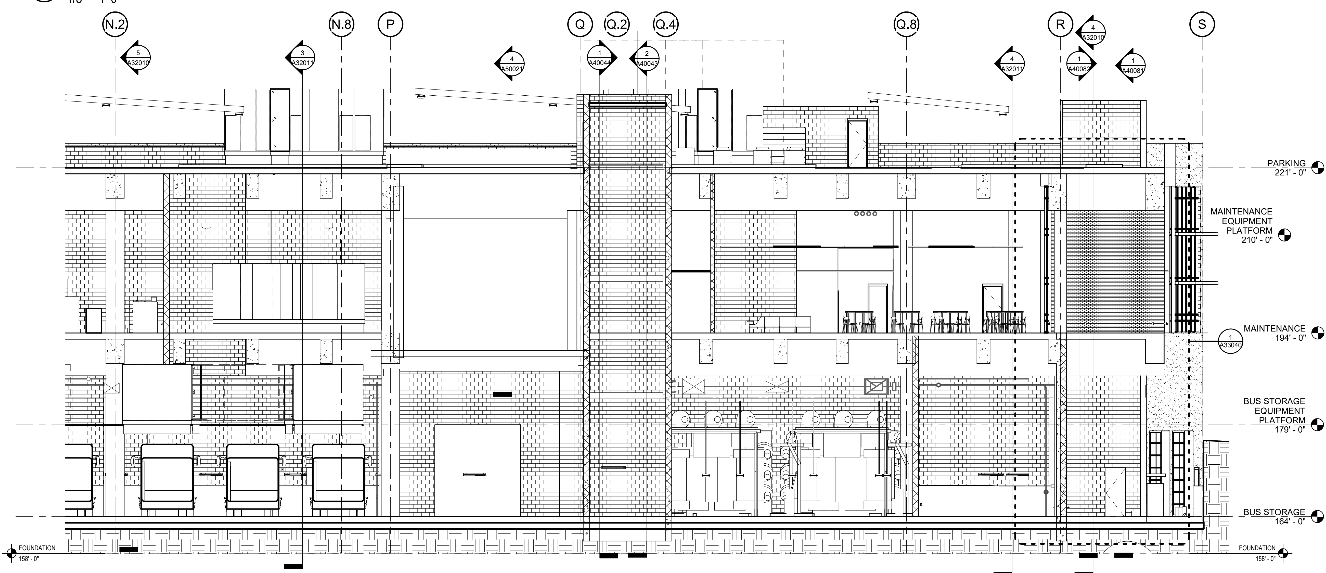
Section 28 - Callout 4 1/8" = 1'-0"
