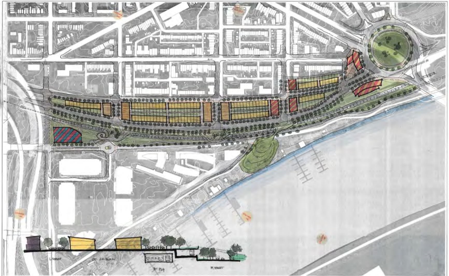
SITE PLAN 1-100 1" = 100'
